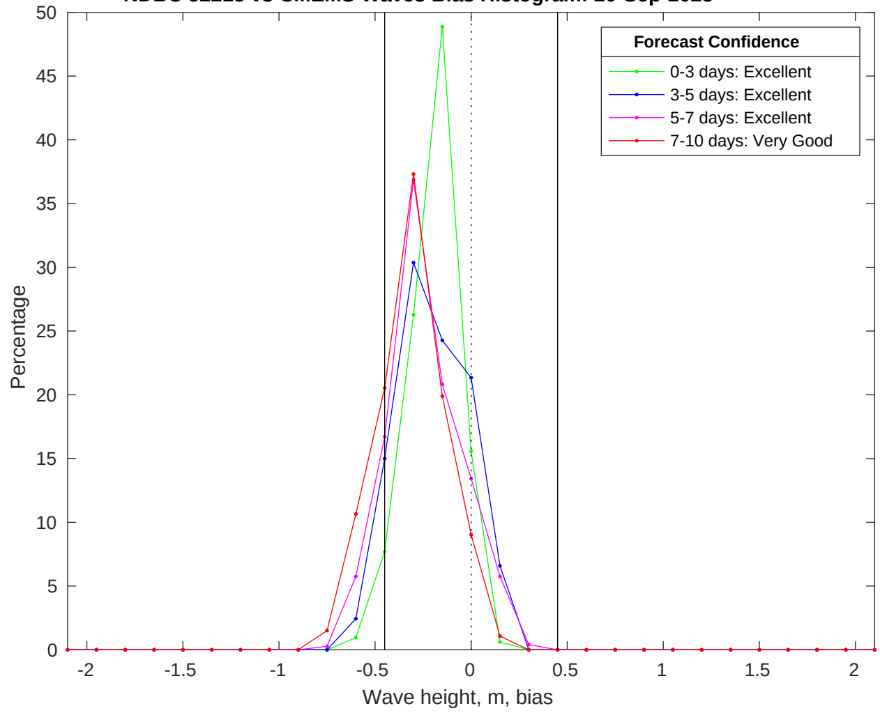
NDBC 52213 vs CMEMS Waves Bias Histogram: 20-Sep-2025
