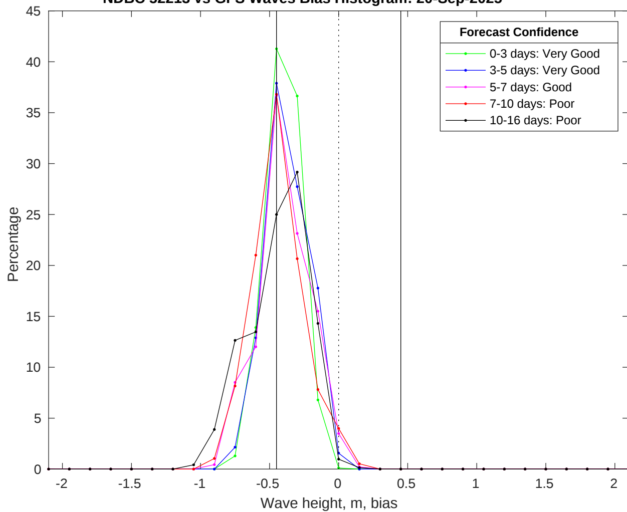
NDBC 52213 vs GFS Waves Bias Histogram: 20-Sep-2025
