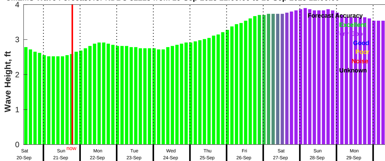
CMEMS Wave Forecast for NDBC 52213 from 19-Sep-2025 11:00:00 to 29-Sep-2025 11:00:00
