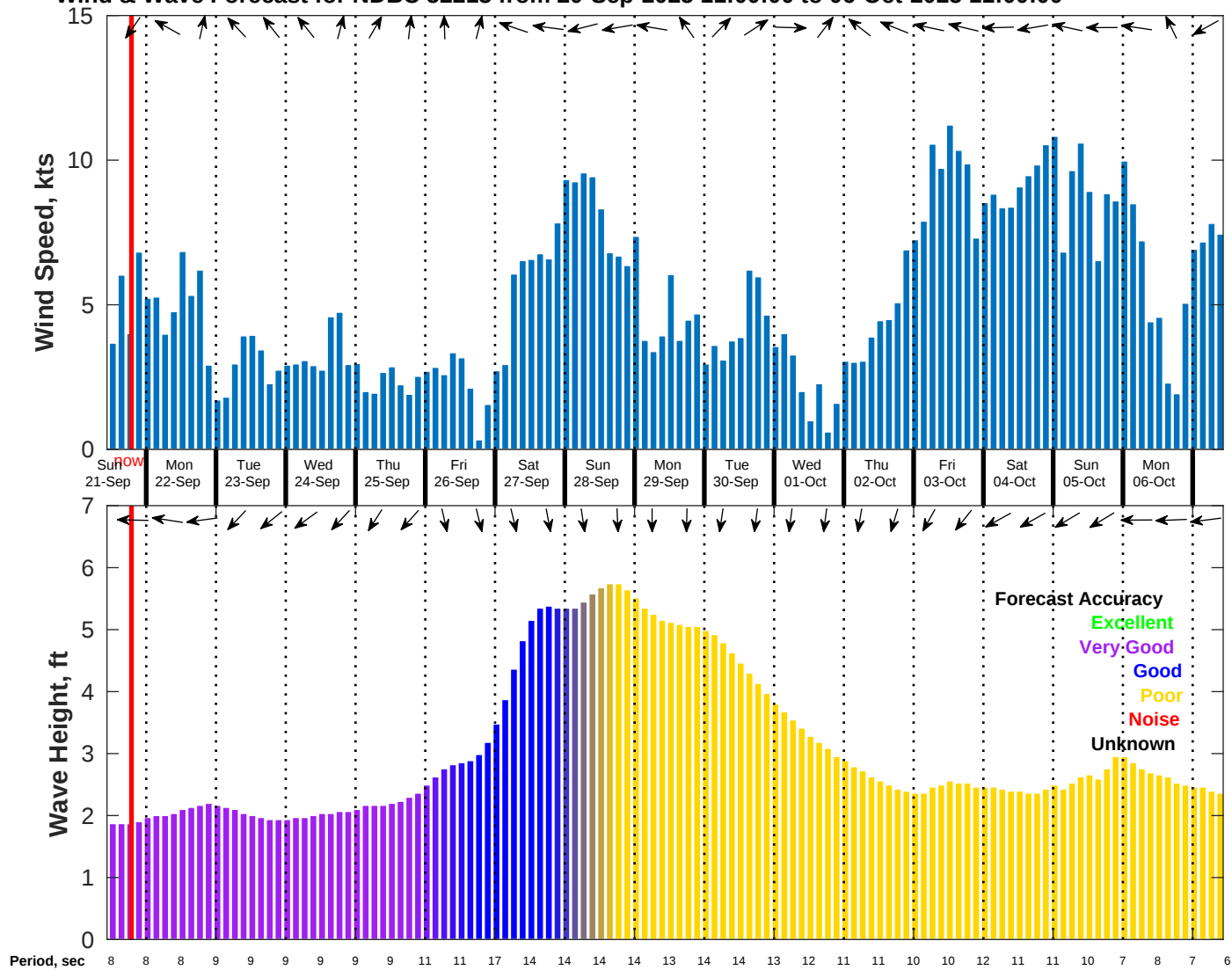
Wind & Wave Forecast for NDBC 52213 from 20-Sep-2025 11:00:00 to 06-Oct-2025 11:00:00
