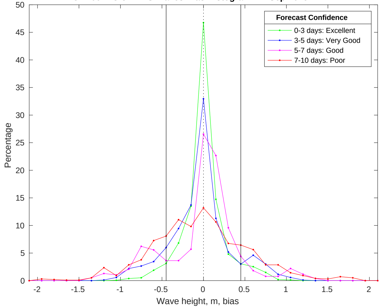
NDBC 41004 vs CMEMS Waves Bias Histogram: 21-Sep-2025
