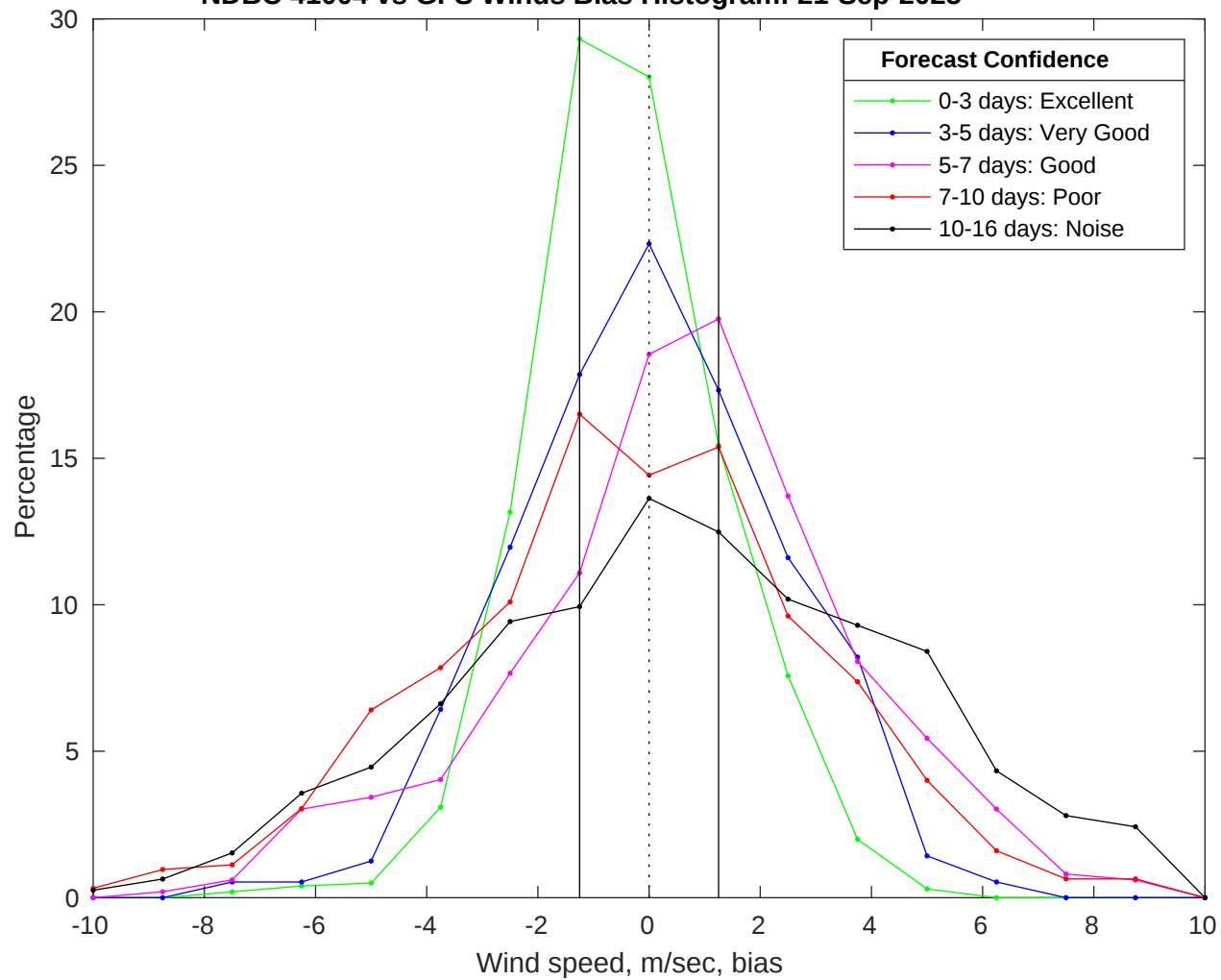
NDBC 41004 vs GFS Winds Bias Histogram: 21-Sep-2025
