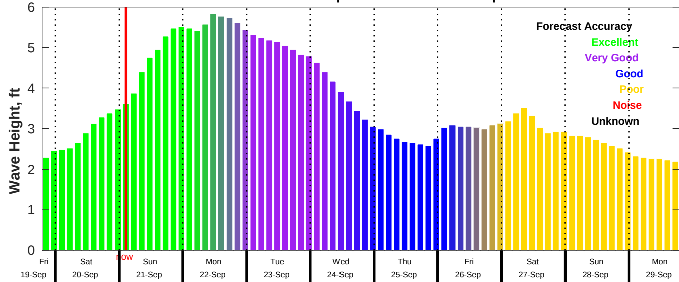
CMEMS Wave Forecast for NDBC 41004 from 19-Sep-2025 19:00:00 to 29-Sep-2025 19:00:00
