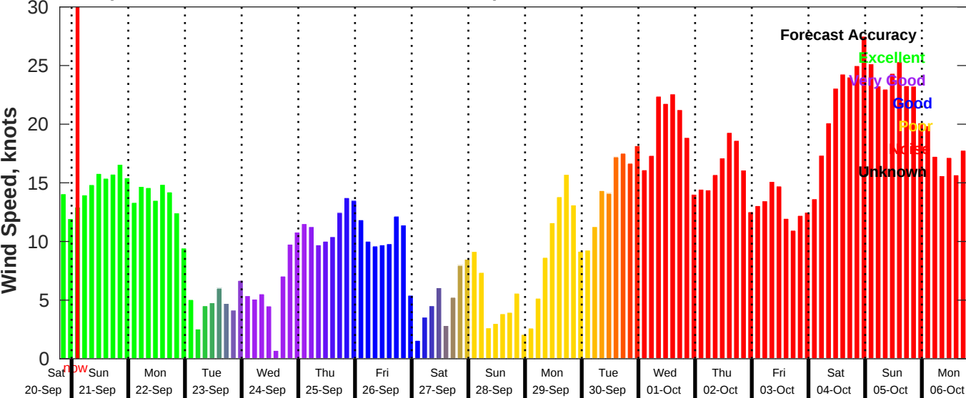
GFS Wind Speed Forecast for NDBC 41004 from 20-Sep-2025 19:00:00 to 06-Oct-2025 19:00:00
