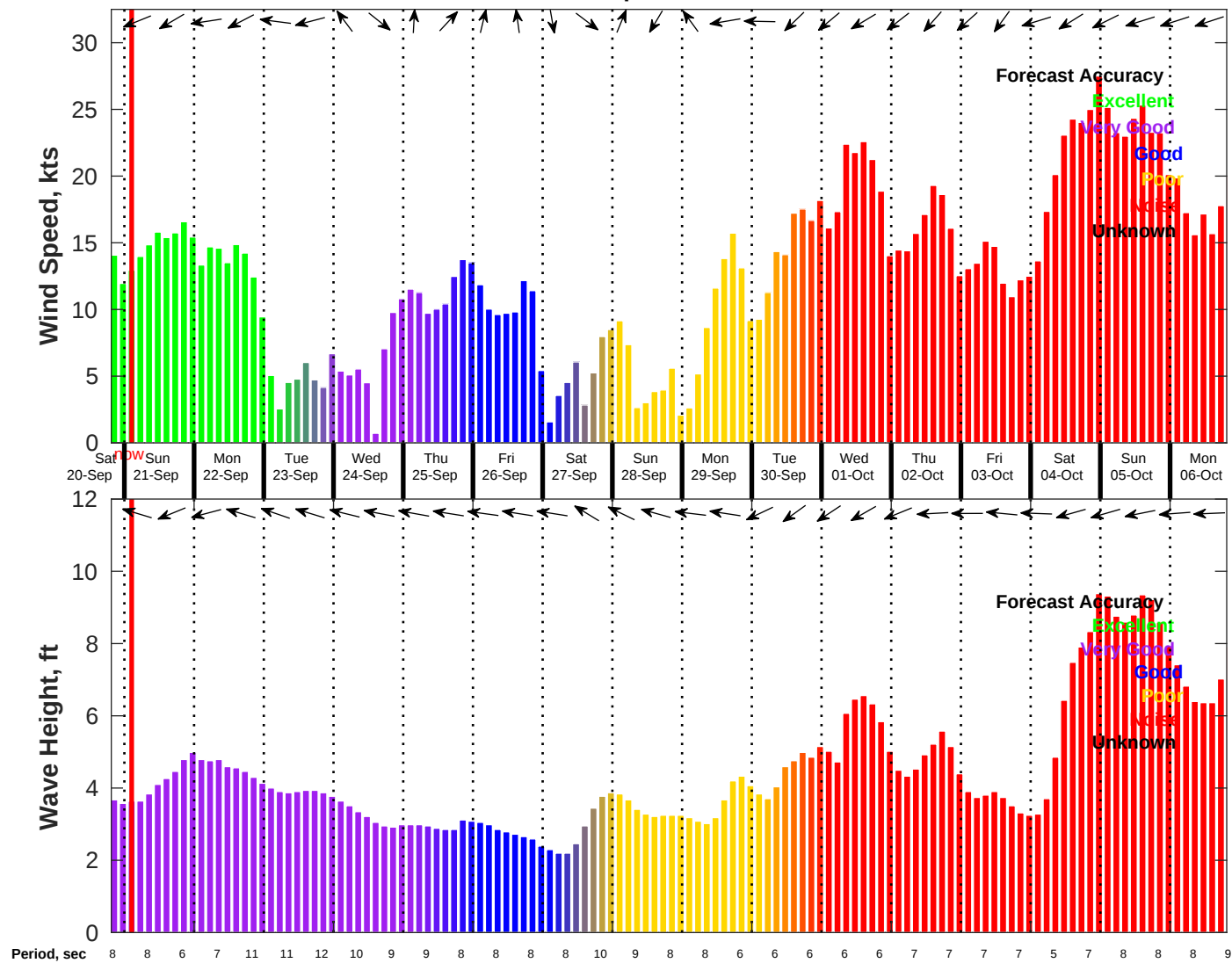
Wind & Wave Forecast for NDBC 41004 from 20-Sep-2025 19:00:00 to 06-Oct-2025 19:00:00
