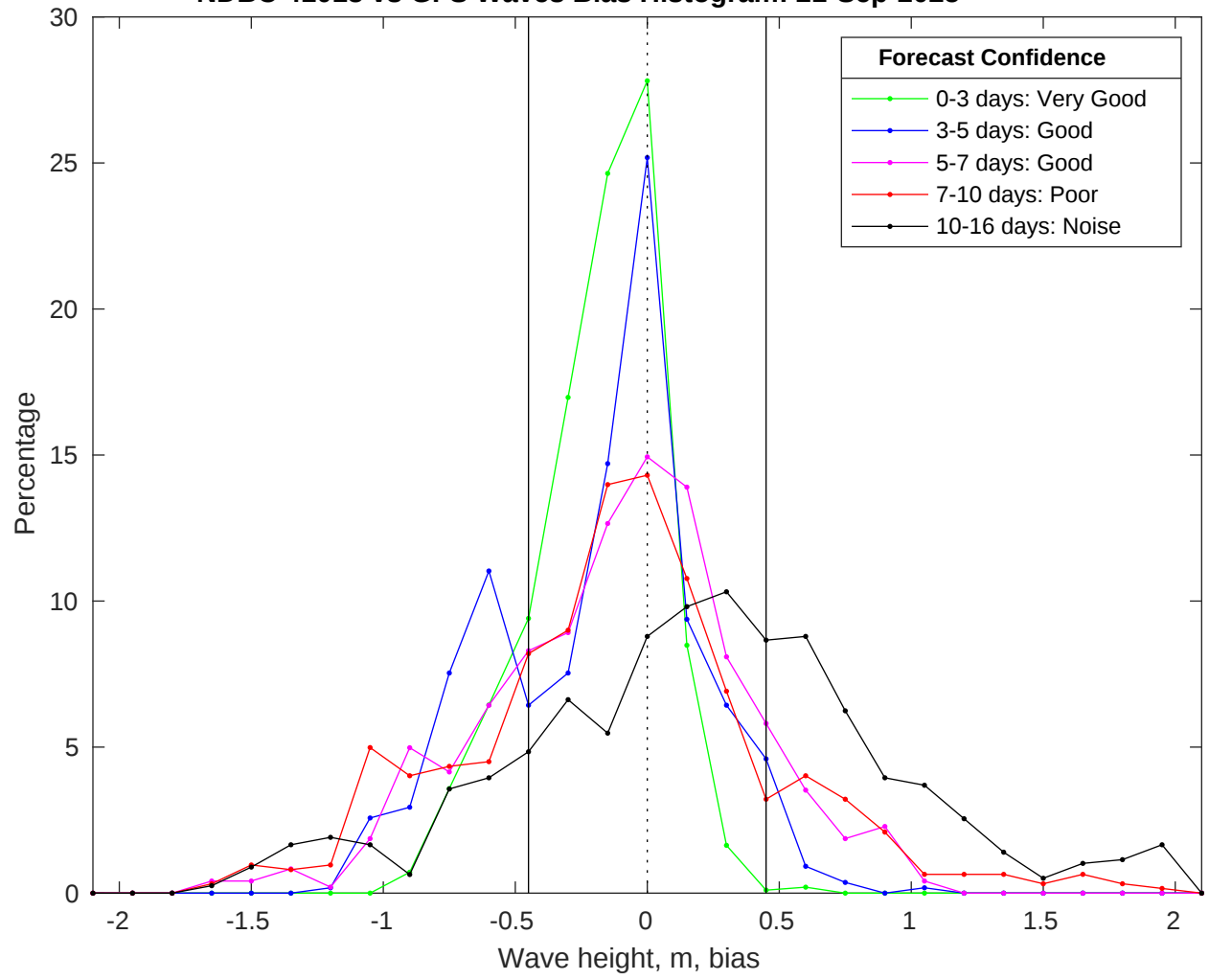
NDBC 41013 vs GFS Waves Bias Histogram: 21-Sep-2025
