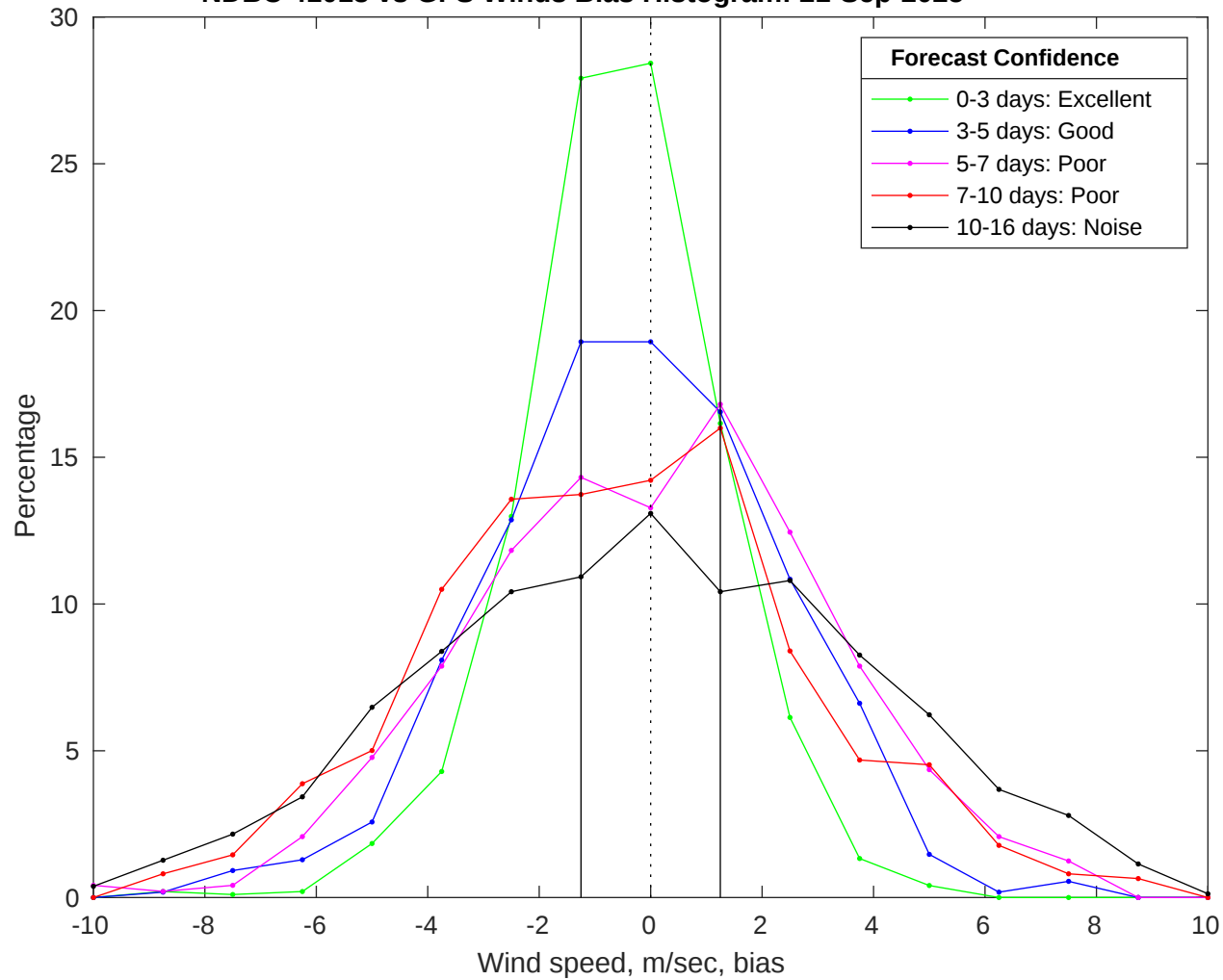
NDBC 41013 vs GFS Winds Bias Histogram: 21-Sep-2025
