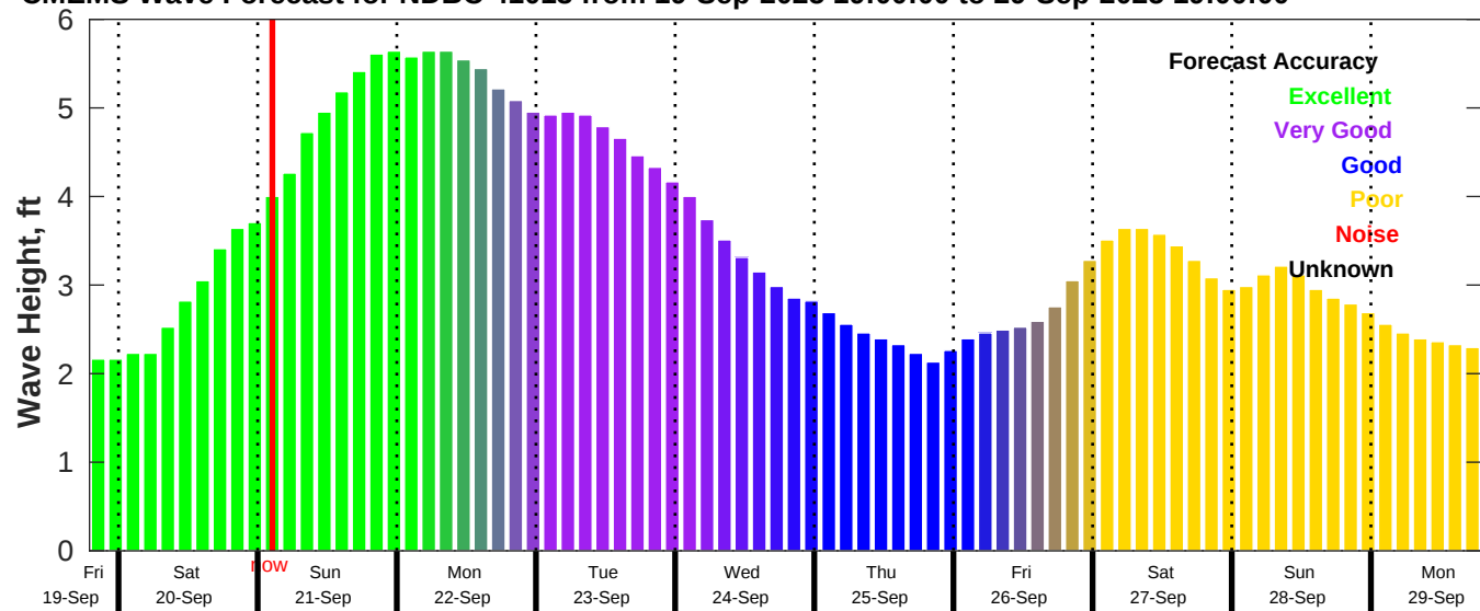
CMEMS Wave Forecast for NDBC 41013 from 19-Sep-2025 19:00:00 to 29-Sep-2025 19:00:00
