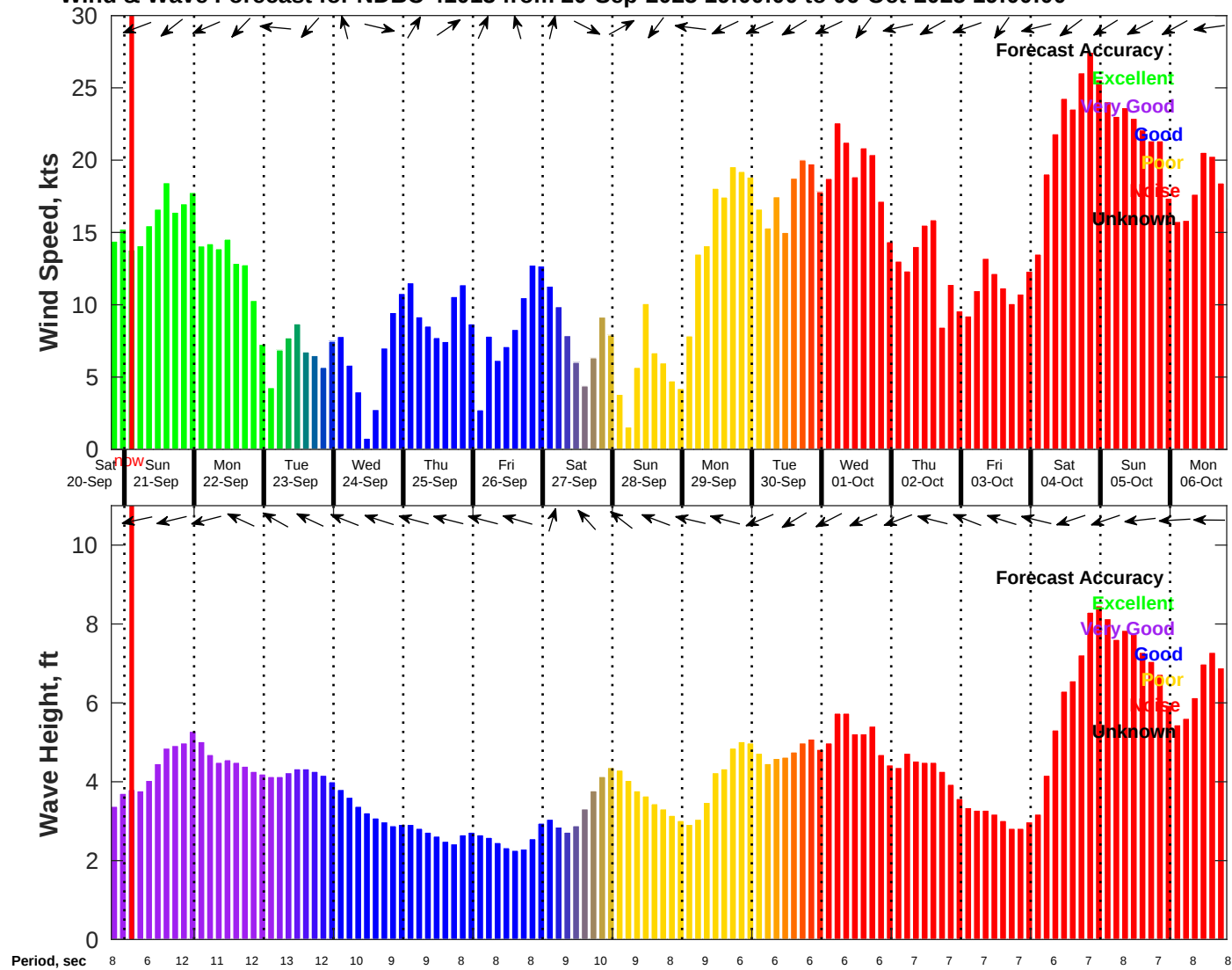
Wind & Wave Forecast for NDBC 41013 from 20-Sep-2025 19:00:00 to 06-Oct-2025 19:00:00
