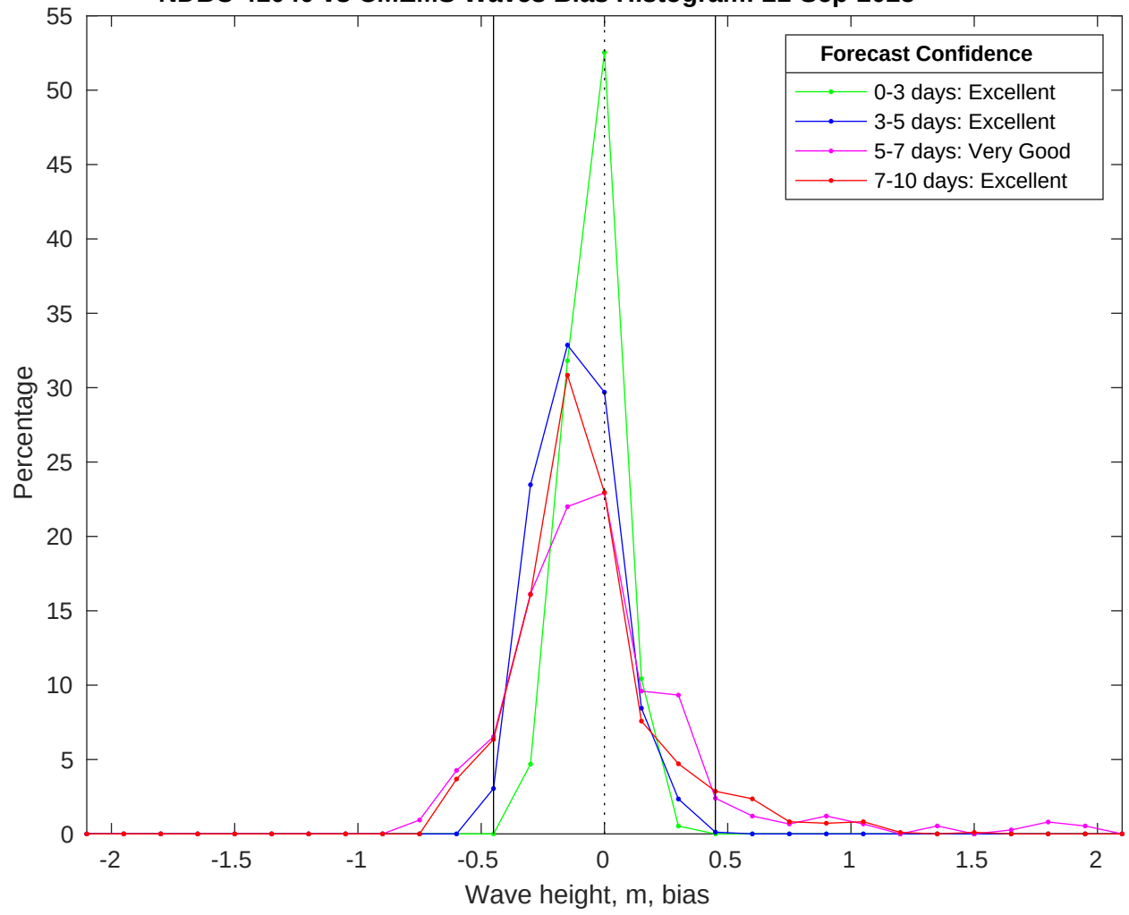
NDBC 41040 vs CMEMS Waves Bias Histogram: 21-Sep-2025
