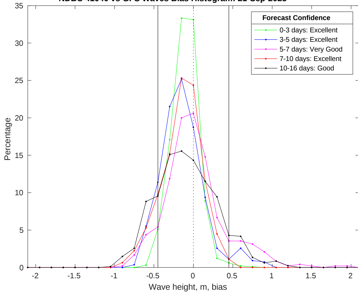
NDBC 41040 vs GFS Waves Bias Histogram: 21-Sep-2025
