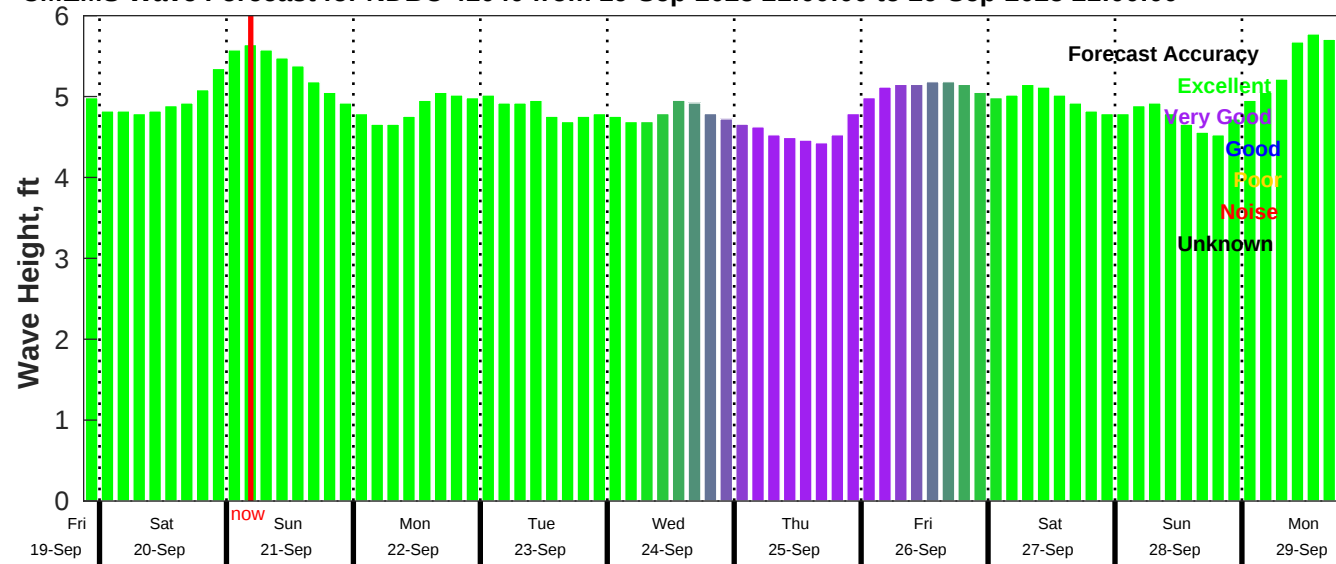
CMEMS Wave Forecast for NDBC 41040 from 19-Sep-2025 21:00:00 to 29-Sep-2025 21:00:00
