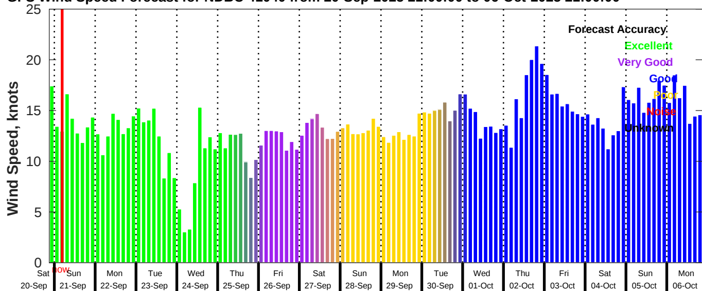
GFS Wind Speed Forecast for NDBC 41040 from 20-Sep-2025 21:00:00 to 06-Oct-2025 21:00:00
