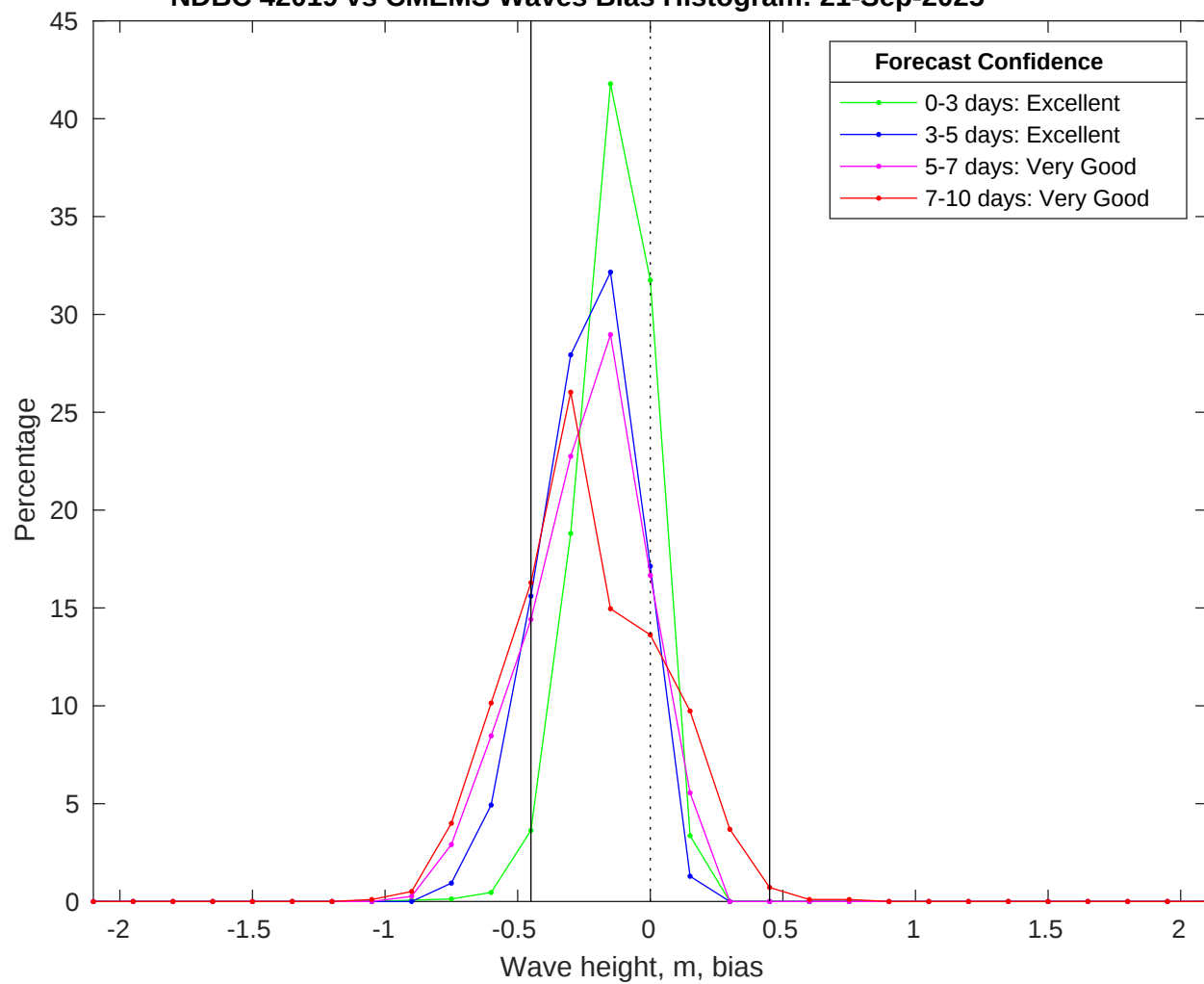
NDBC 42019 vs CMEMS Waves Bias Histogram: 21-Sep-2025
