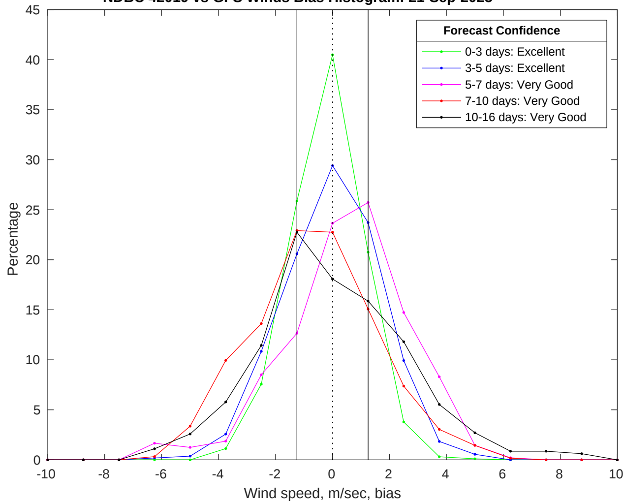
NDBC 42019 vs GFS Winds Bias Histogram: 21-Sep-2025
