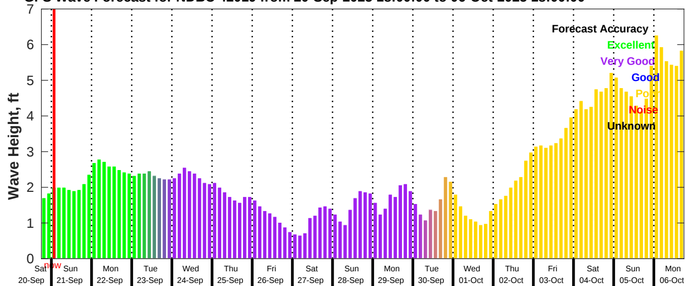
GFS Wave Forecast for NDBC 42019 from 20-Sep-2025 18:00:00 to 06-Oct-2025 18:00:00
