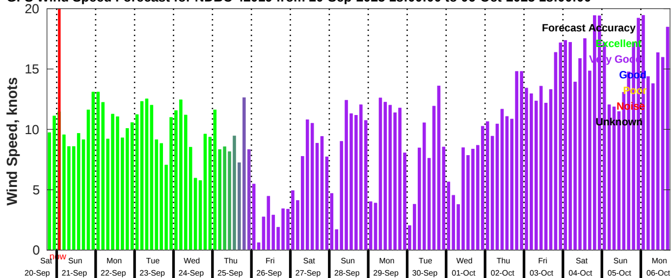
GFS Wind Speed Forecast for NDBC 42019 from 20-Sep-2025 18:00:00 to 06-Oct-2025 18:00:00
