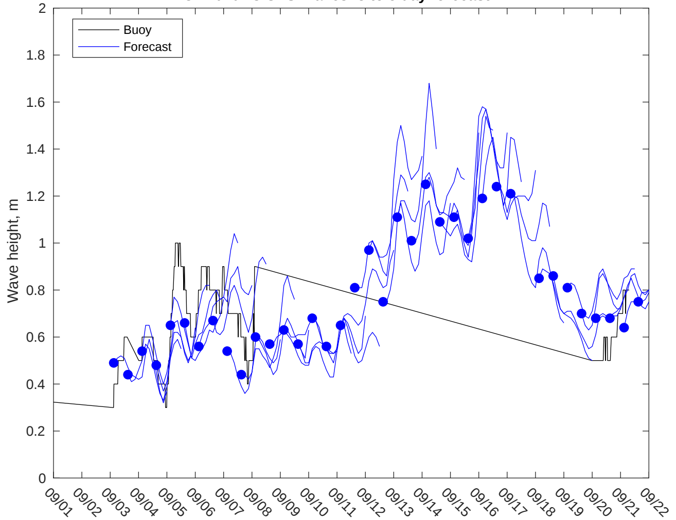
NDBC 42020 vs GFS Waves: 3 to 5 day forecast
