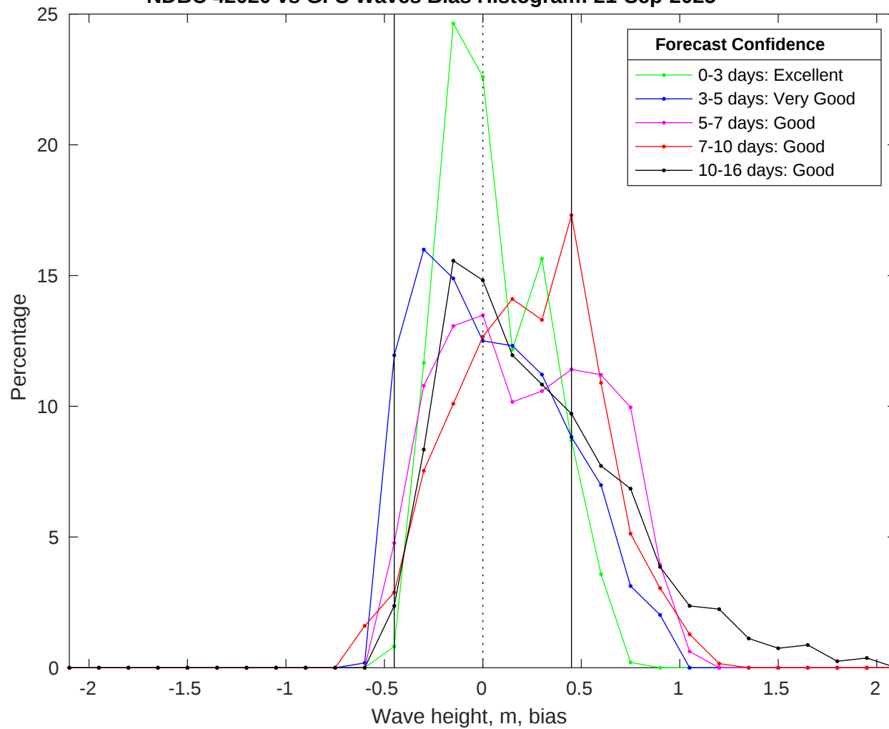
NDBC 42020 vs GFS Waves Bias Histogram: 21-Sep-2025
