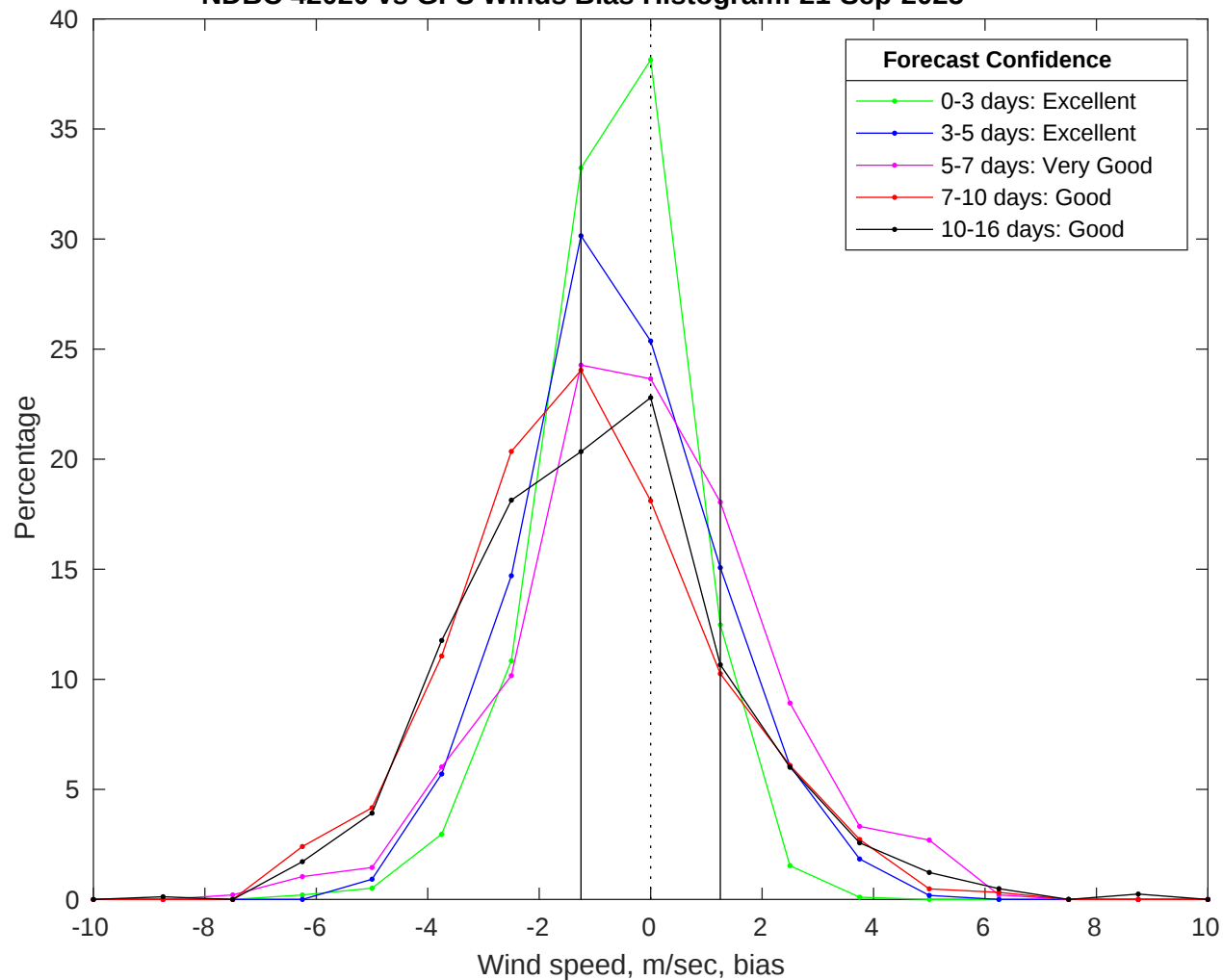
NDBC 42020 vs GFS Winds Bias Histogram: 21-Sep-2025
