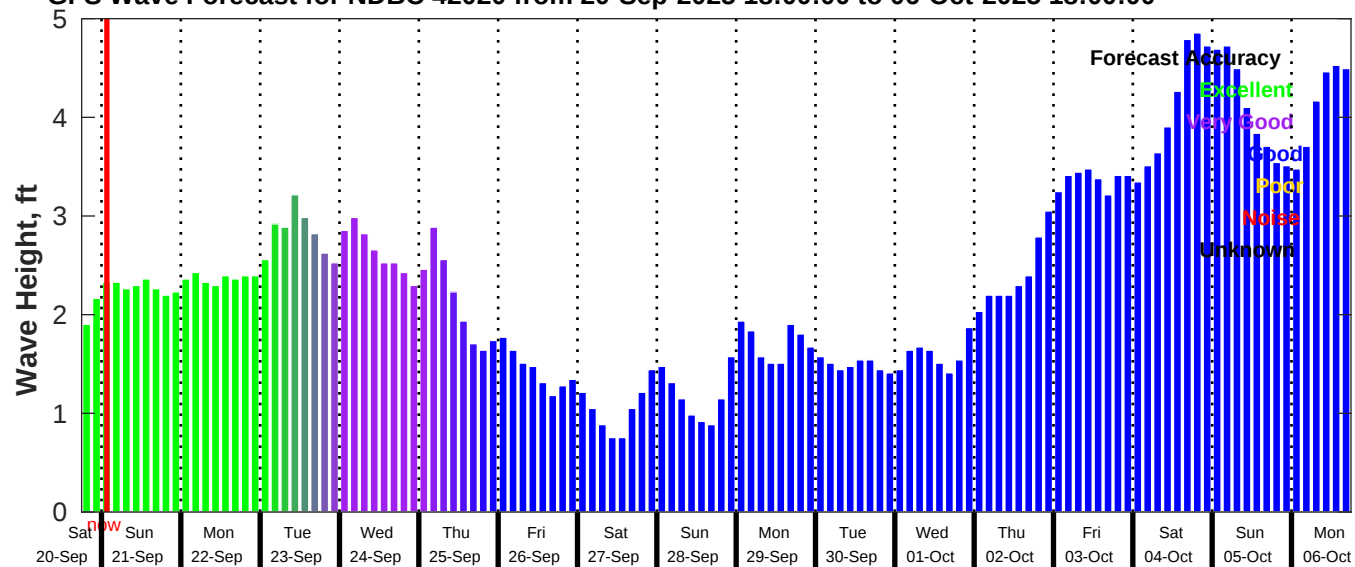
GFS Wave Forecast for NDBC 42020 from 20-Sep-2025 18:00:00 to 06-Oct-2025 18:00:00
