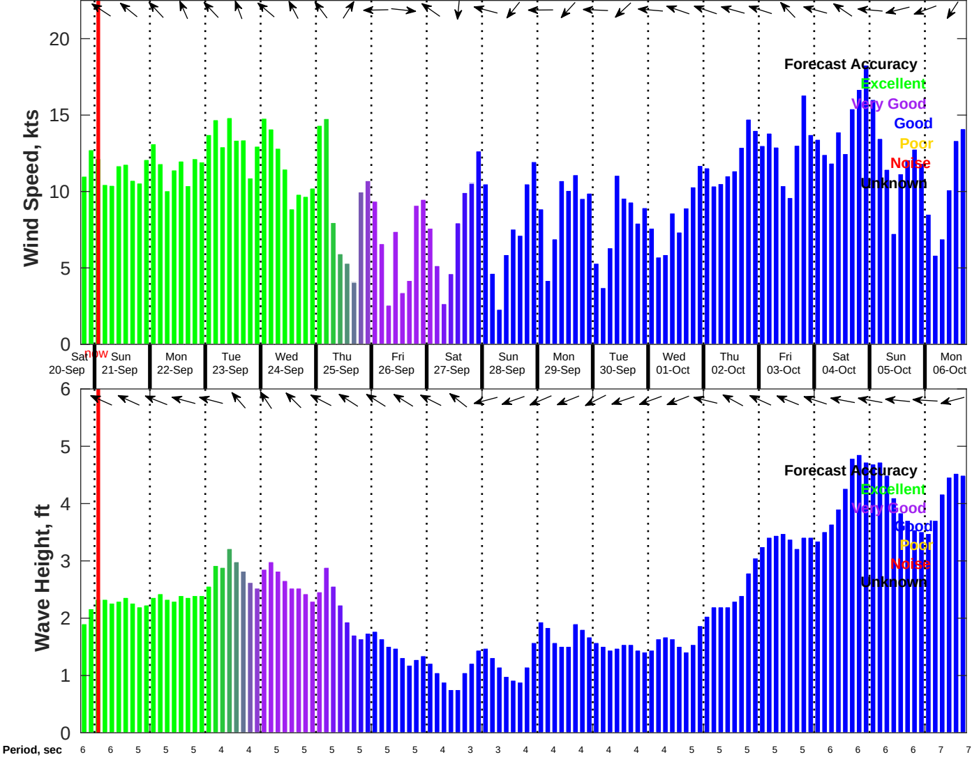
Wind & Wave Forecast for NDBC 42020 from 20-Sep-2025 18:00:00 to 06-Oct-2025 18:00:00
