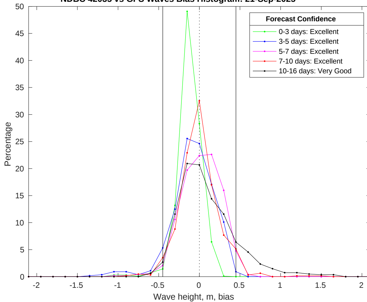
NDBC 42035 vs GFS Waves Bias Histogram: 21-Sep-2025
