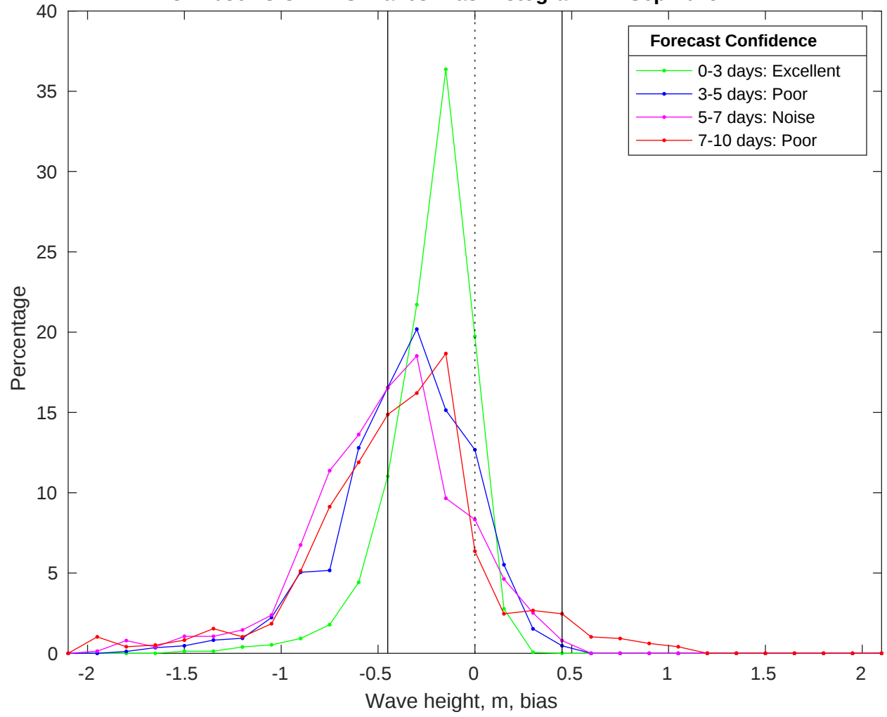
NDBC 42036 vs CMEMS Waves Bias Histogram: 21-Sep-2025
