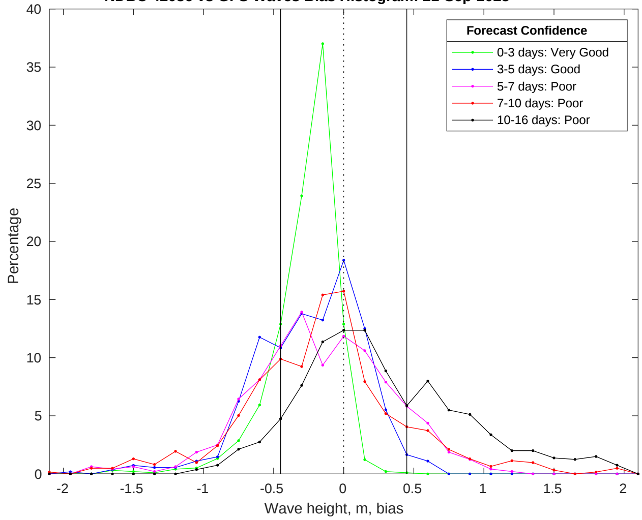
NDBC 42036 vs GFS Waves Bias Histogram: 21-Sep-2025
