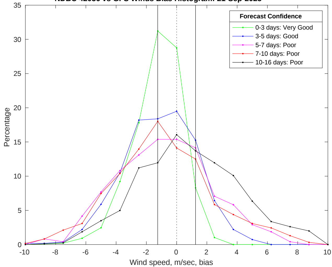
NDBC 42036 vs GFS Winds Bias Histogram: 21-Sep-2025
