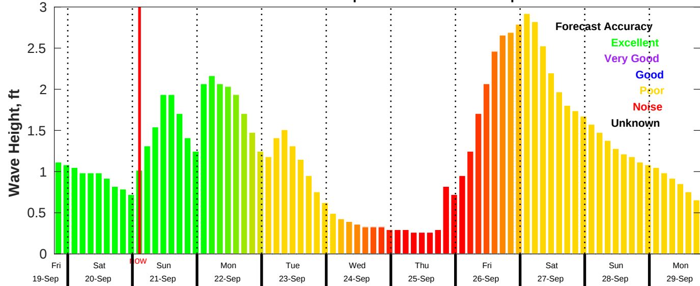
CMEMS Wave Forecast for NDBC 42036 from 19-Sep-2025 19:00:00 to 29-Sep-2025 19:00:00
