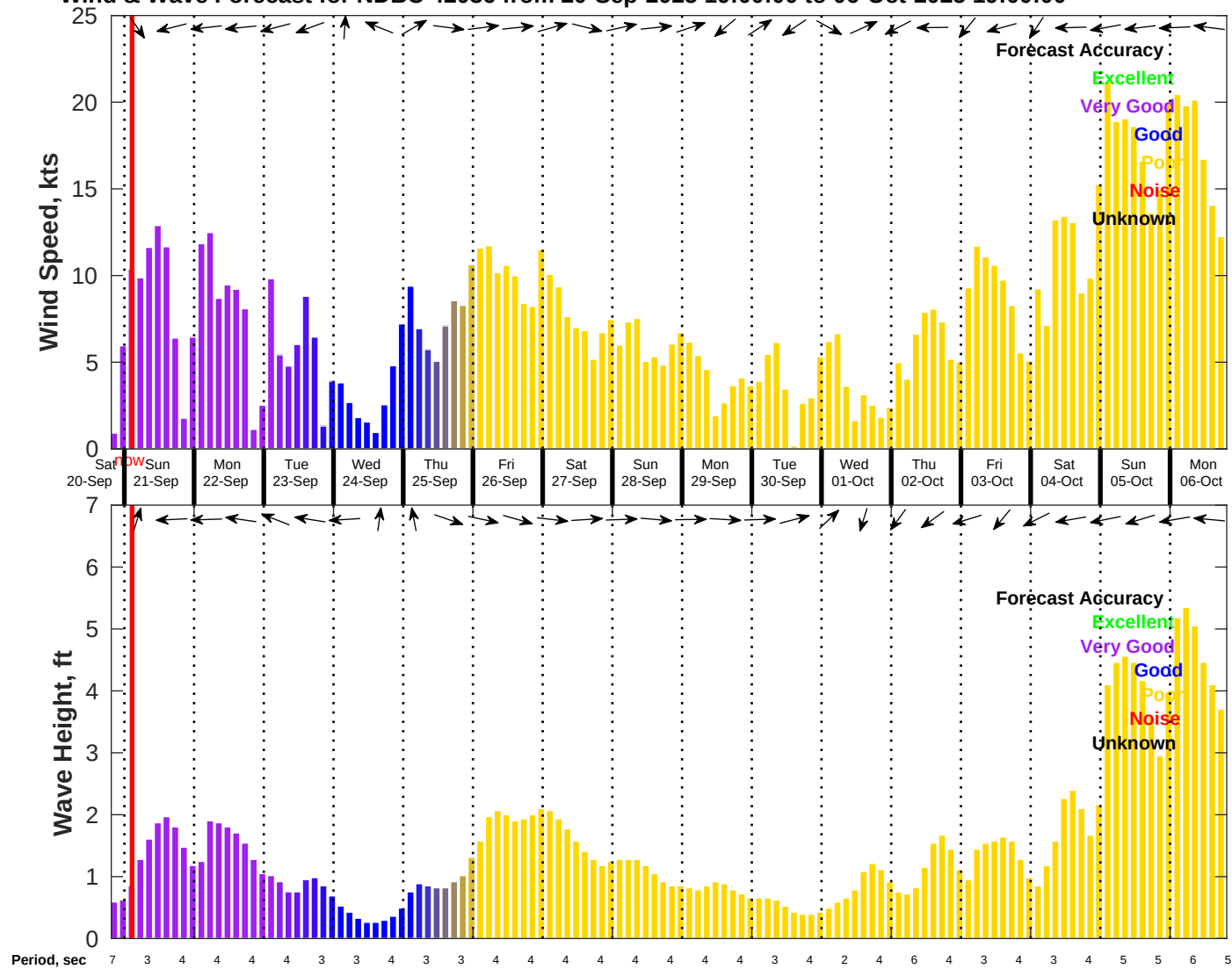
Wind & Wave Forecast for NDBC 42036 from 20-Sep-2025 19:00:00 to 06-Oct-2025 19:00:00
