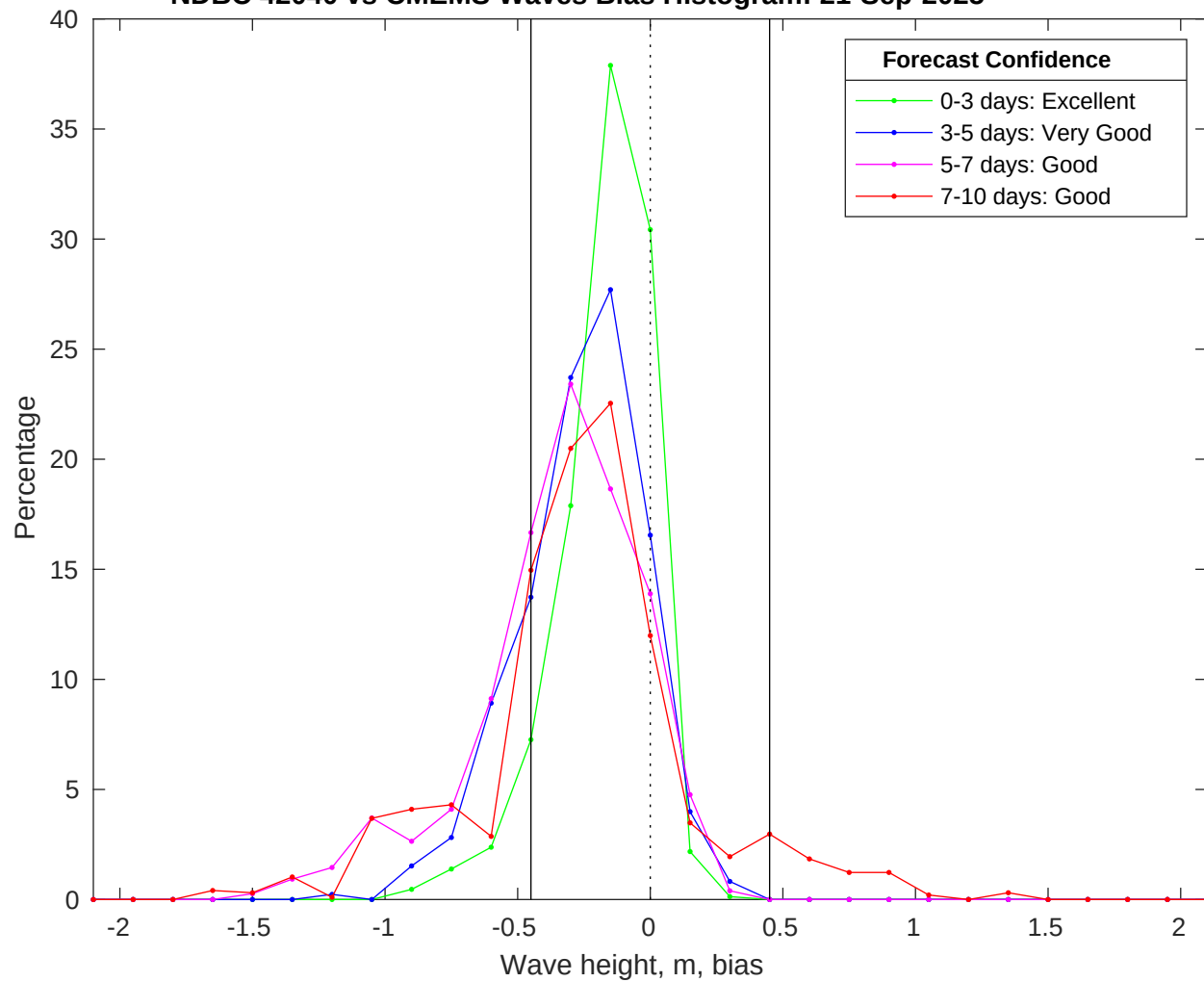
NDBC 42040 vs CMEMS Waves Bias Histogram: 21-Sep-2025
