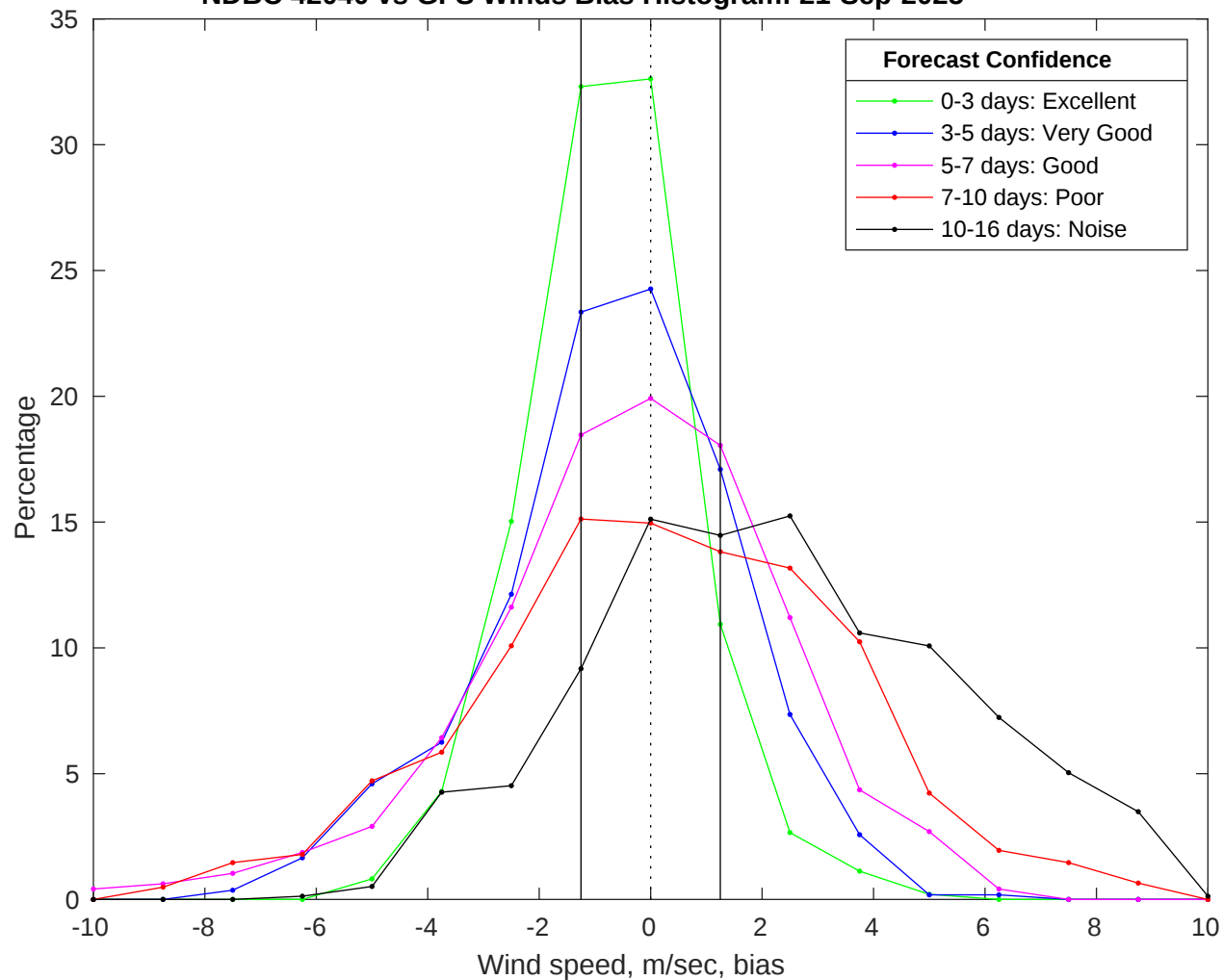
NDBC 42040 vs GFS Winds Bias Histogram: 21-Sep-2025
