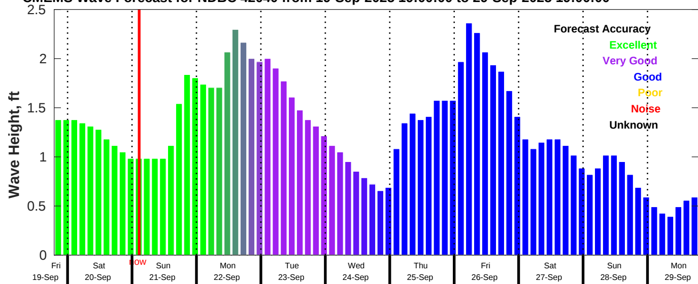
CMEMS Wave Forecast for NDBC 42040 from 19-Sep-2025 19:00:00 to 29-Sep-2025 19:00:00
