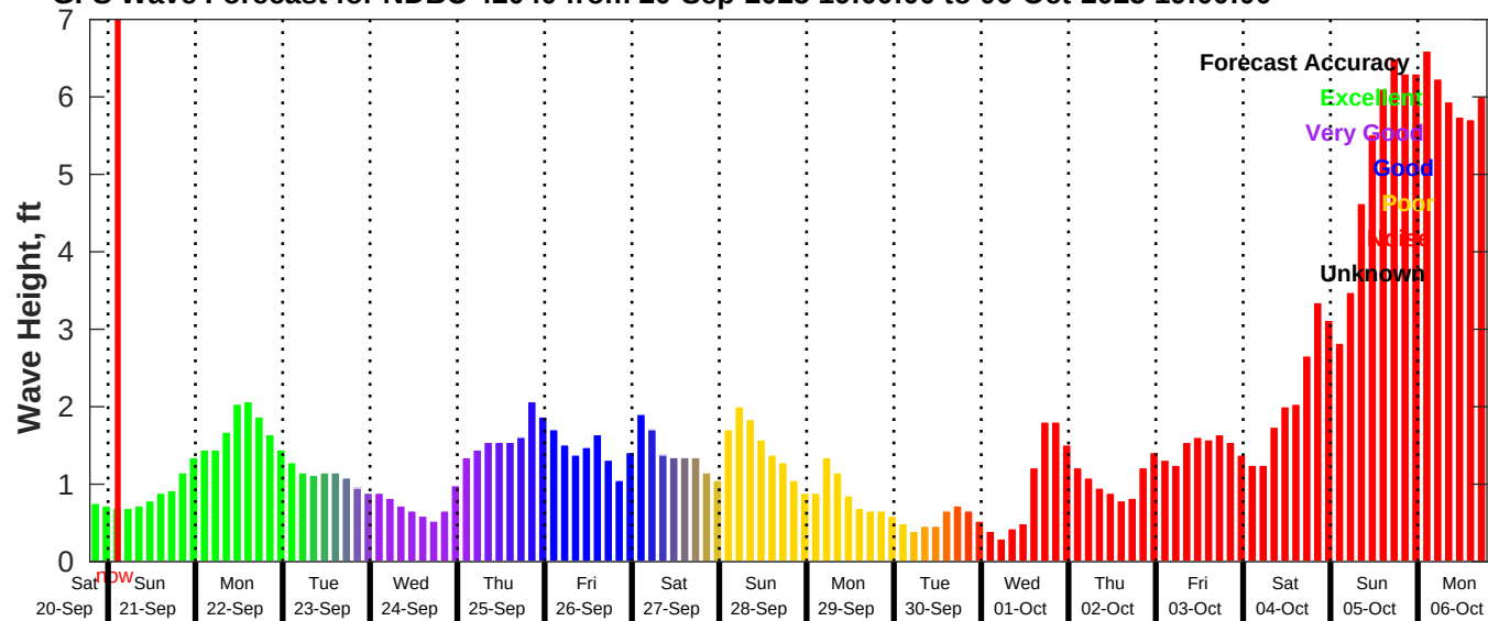
GFS Wave Forecast for NDBC 42040 from 20-Sep-2025 19:00:00 to 06-Oct-2025 19:00:00
