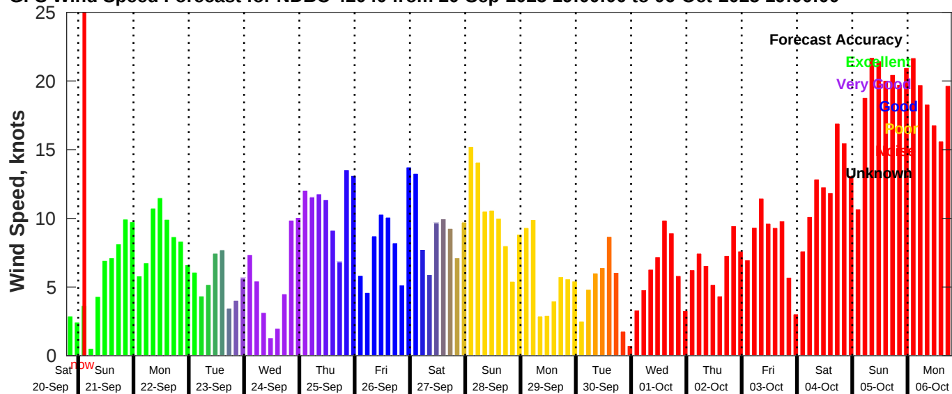
GFS Wind Speed Forecast for NDBC 42040 from 20-Sep-2025 19:00:00 to 06-Oct-2025 19:00:00
