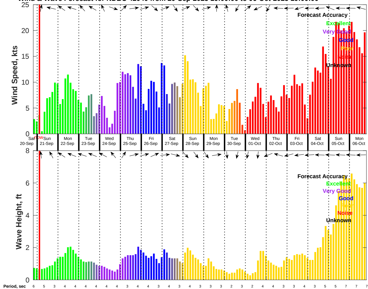
Wind & Wave Forecast for NDBC 42040 from 20-Sep-2025 19:00:00 to 06-Oct-2025 19:00:00
