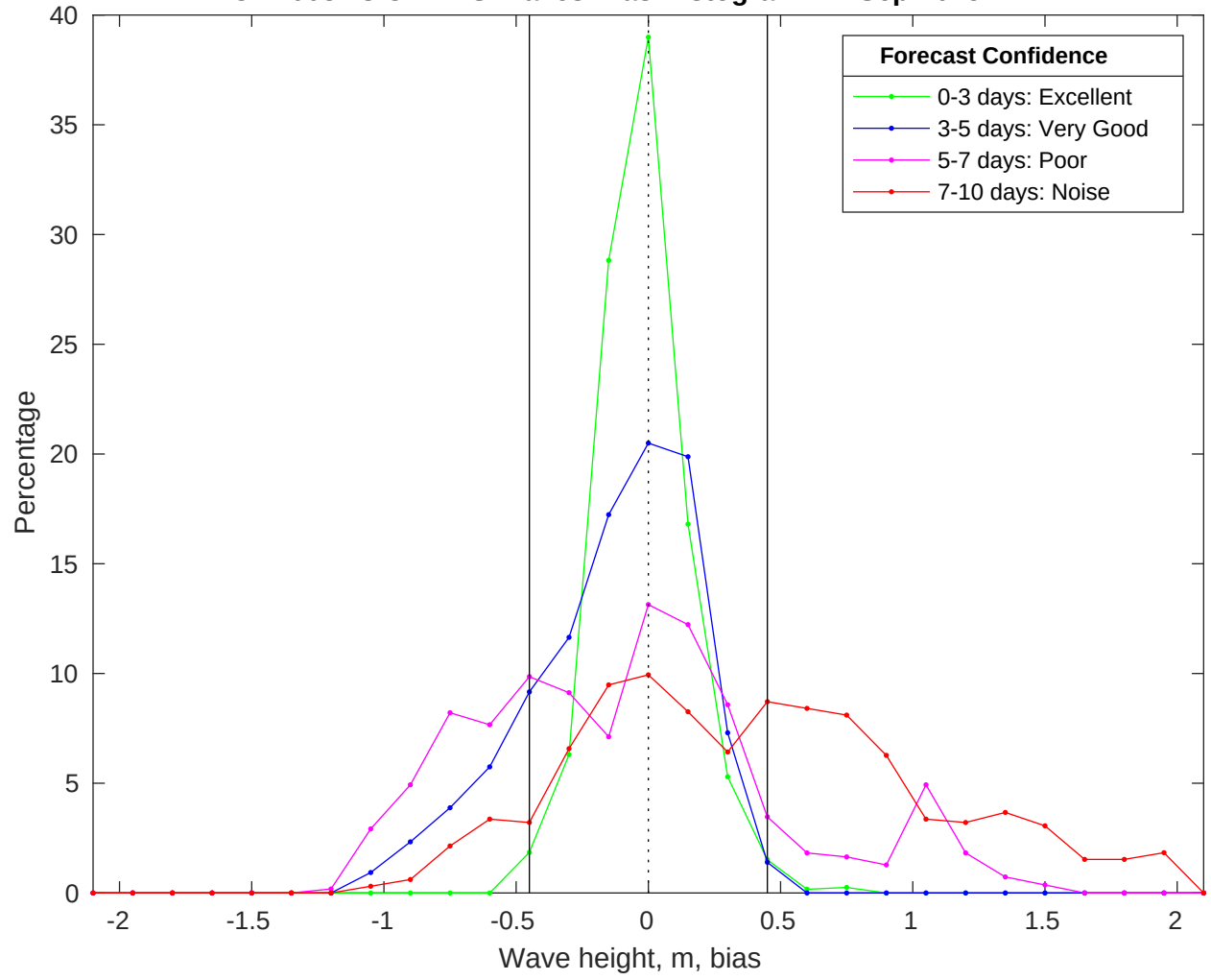
NDBC 44008 vs CMEMS Waves Bias Histogram: 21-Sep-2025
