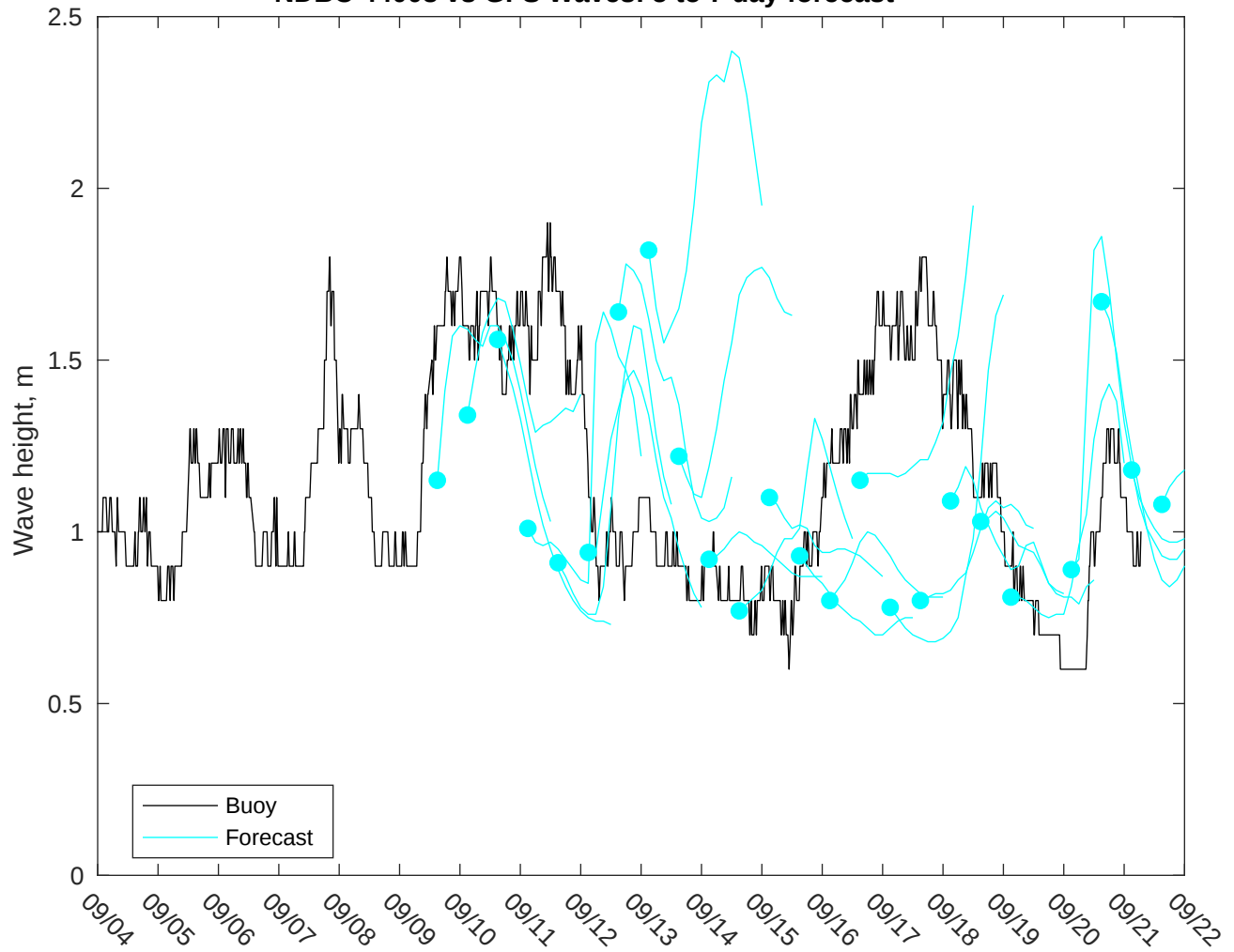
NDBC 44008 vs GFS Waves: 5 to 7 day forecast
