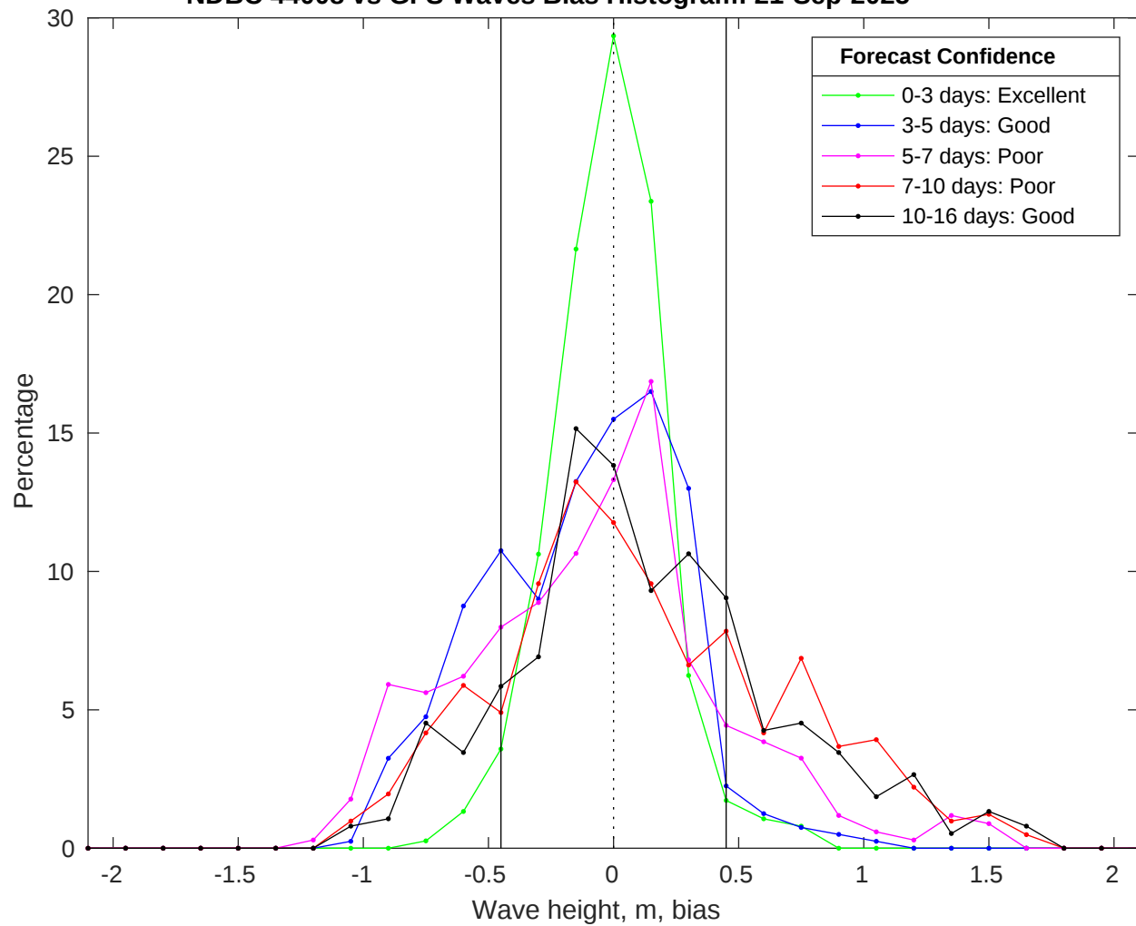
NDBC 44008 vs GFS Waves Bias Histogram: 21-Sep-2025
