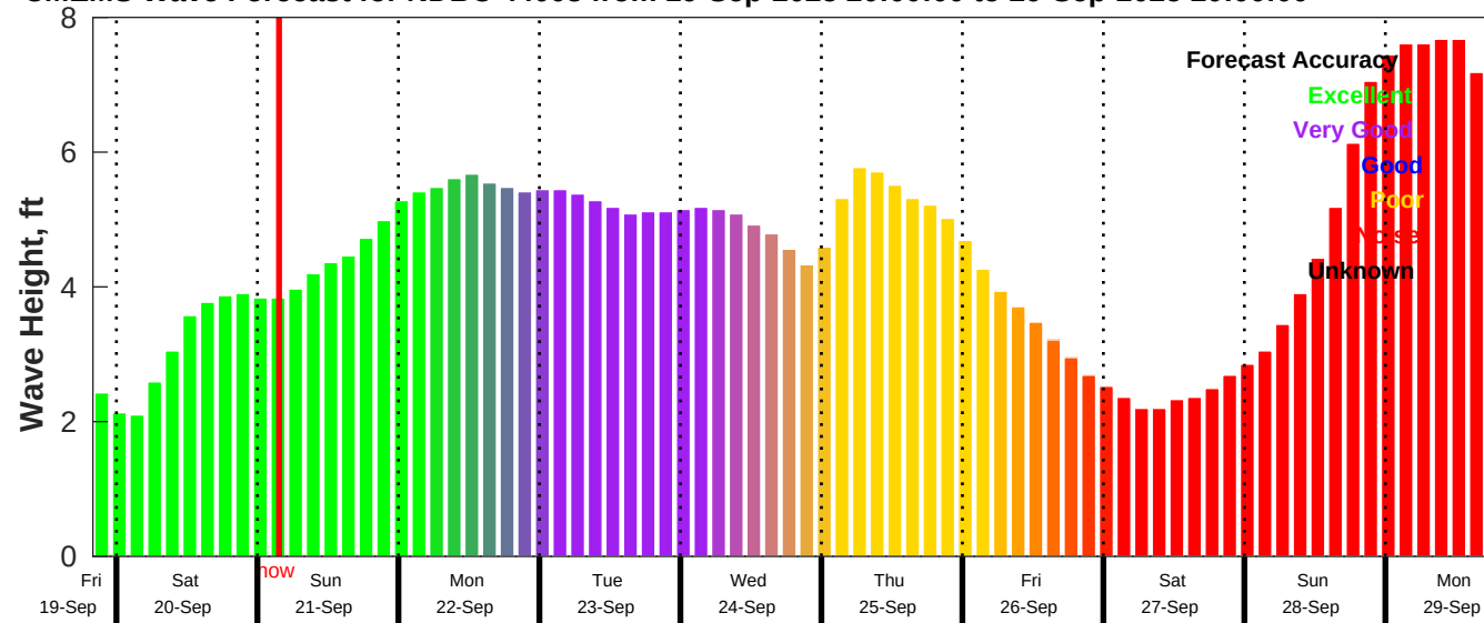
CMEMS Wave Forecast for NDBC 44008 from 19-Sep-2025 20:00:00 to 29-Sep-2025 20:00:00
