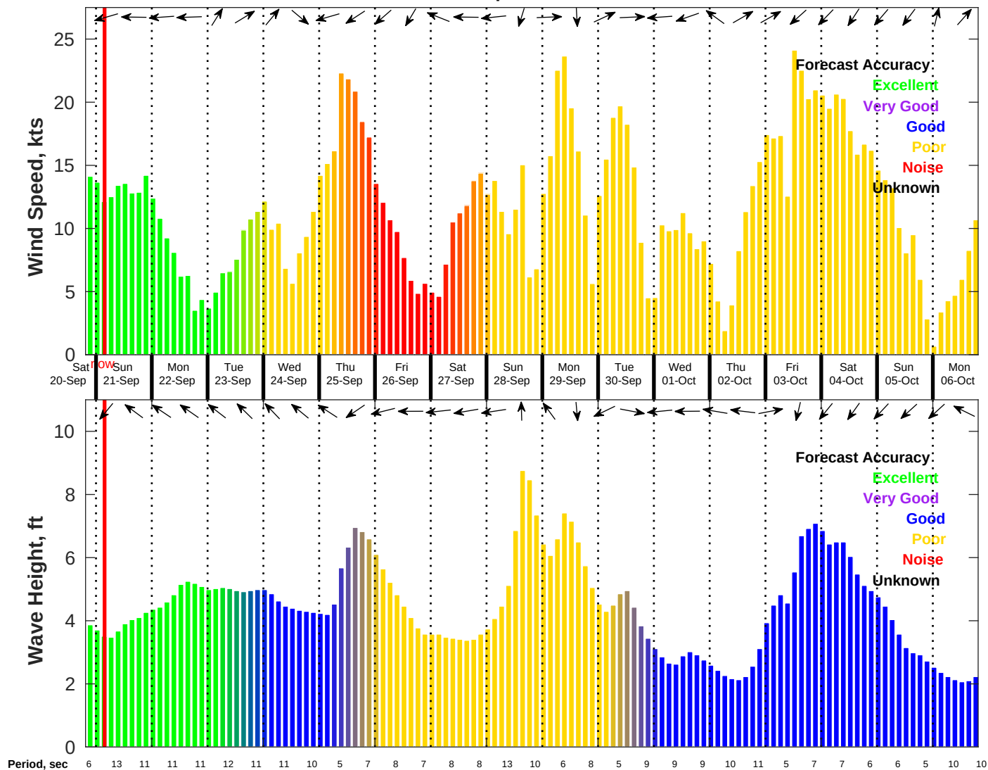
Wind & Wave Forecast for NDBC 44008 from 20-Sep-2025 20:00:00 to 06-Oct-2025 20:00:00
