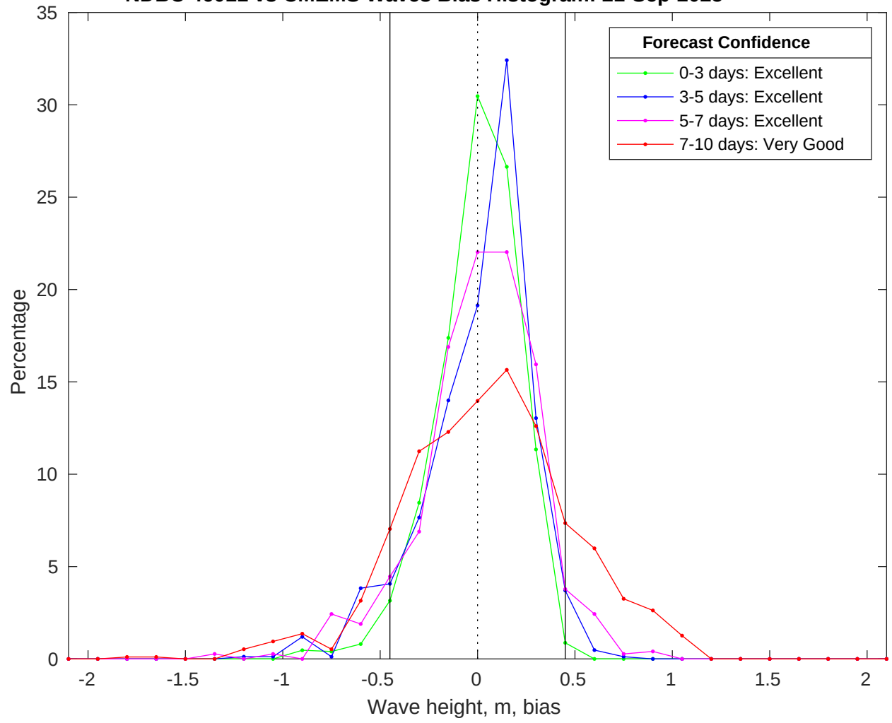
NDBC 46011 vs CMEMS Waves Bias Histogram: 21-Sep-2025
