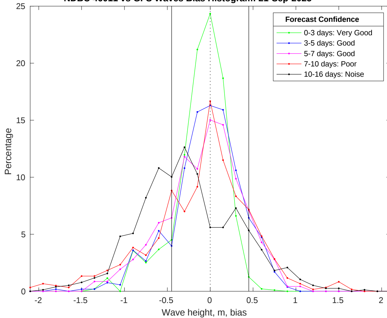
NDBC 46011 vs GFS Waves Bias Histogram: 21-Sep-2025
