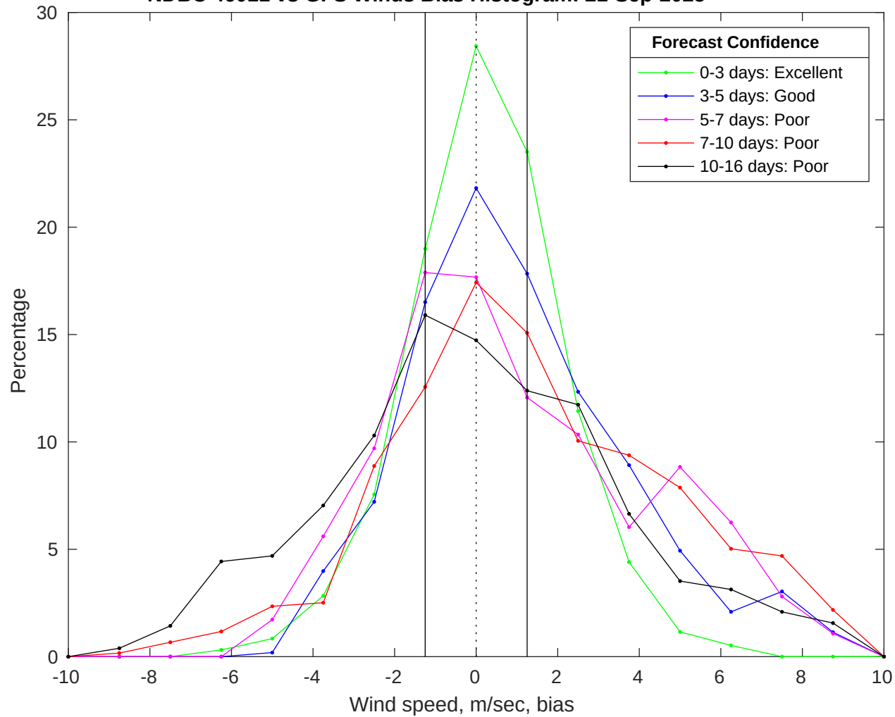
NDBC 46011 vs GFS Winds Bias Histogram: 21-Sep-2025
