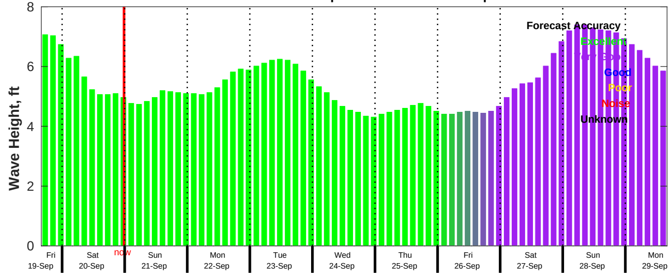
CMEMS Wave Forecast for NDBC 46011 from 19-Sep-2025 16:00:00 to 29-Sep-2025 16:00:00
