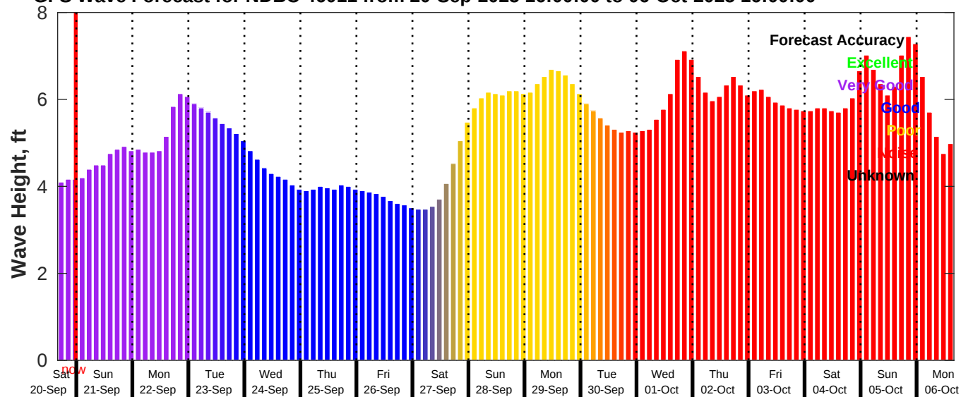
GFS Wave Forecast for NDBC 46011 from 20-Sep-2025 16:00:00 to 06-Oct-2025 16:00:00
