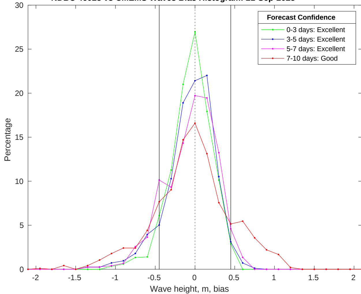
NDBC 46028 vs CMEMS Waves Bias Histogram: 21-Sep-2025
