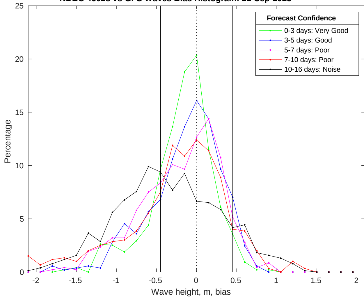
NDBC 46028 vs GFS Waves Bias Histogram: 21-Sep-2025
